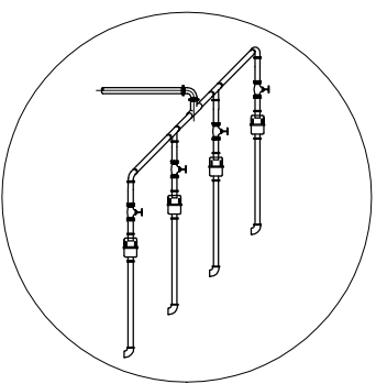
HORIZONTAL INSTALLATION (ALTERNATIVE)
